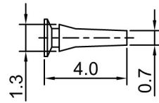
POLARIZING PLUG
