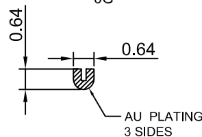
SECTION Y-Y SCALE 8:1
