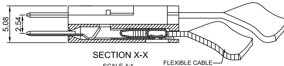
SECTION X-X SCALE 4:1
