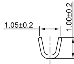
B-B SECTION
