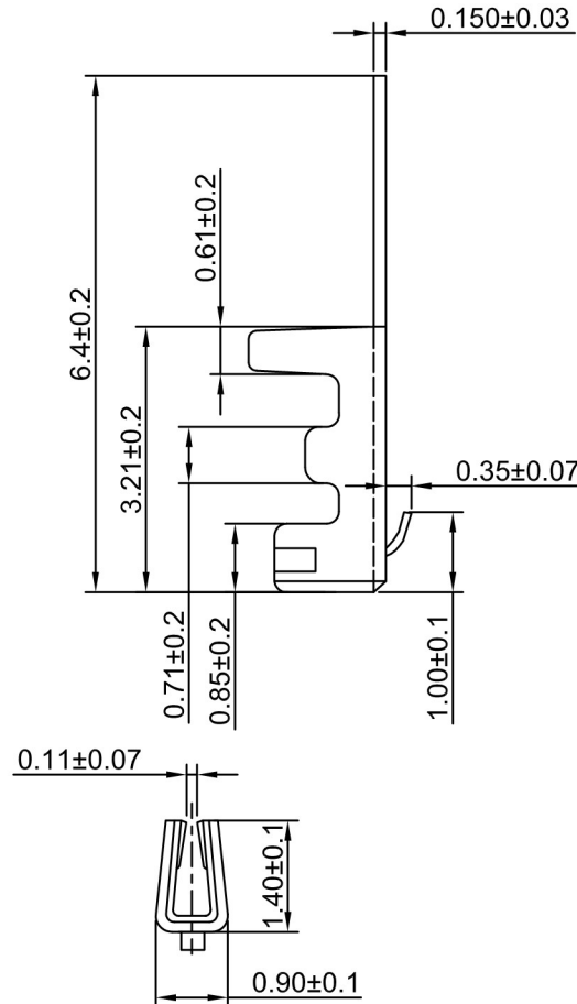
C-C SECTION
