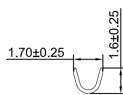
C-C SECTION
