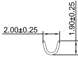
B-B SECTION
