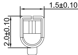
C-C SECTION
