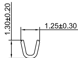
B-B SECTION
