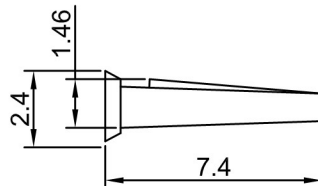
HOUSING POLARIZING KEY
