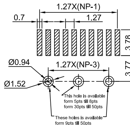
P.C.B LAYOUT (PCB BOARD TOLERANCE±0.05)
