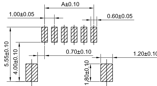
Recommnded P.C.B Layout
