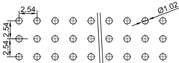
PCB LAYOUT
