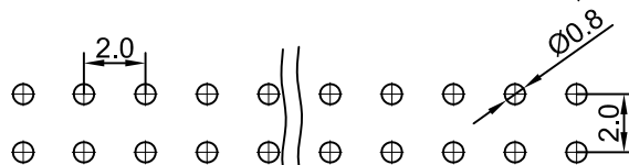
PCB LAYOUT
