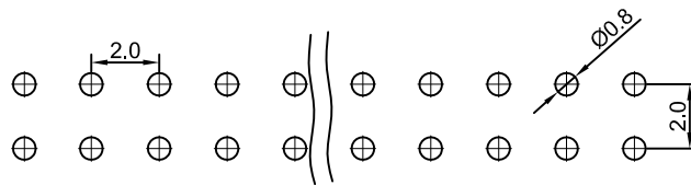
PCB LAYOUT
