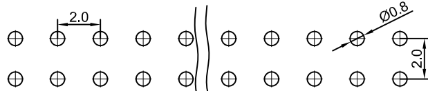
PCB LAYOUT
