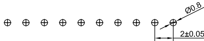
PCB LAYOUT
