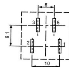
relay outline dimensions
