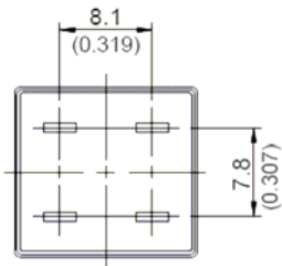
relay outline
