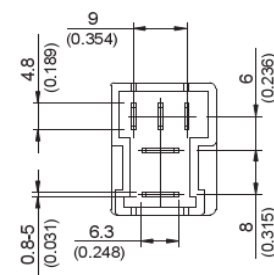
relay outline dimensions
